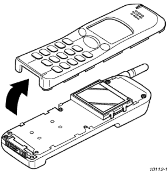
Figure 4.2: Case Disassembly
