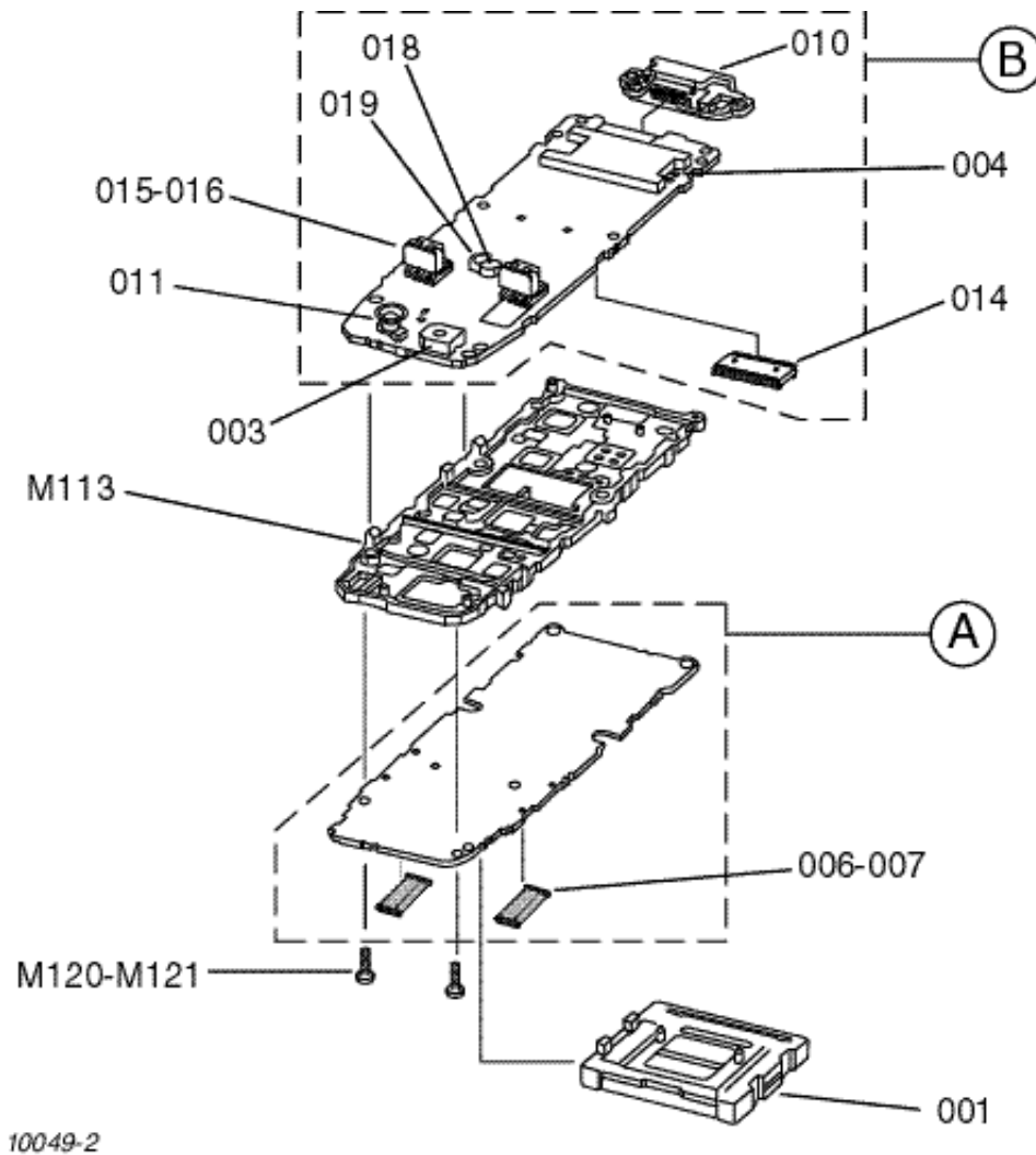
Figure 9.3: GD30/GD50 Sub-Assemblies
