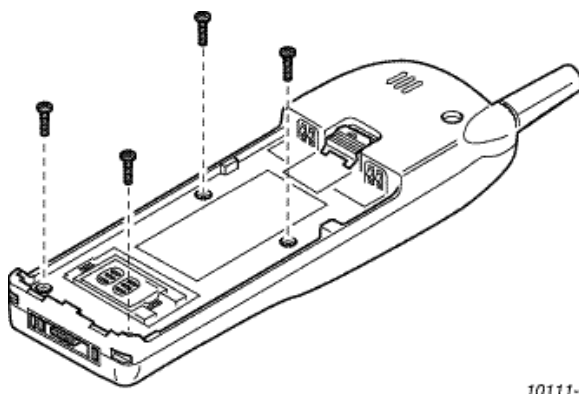
Figure 4.1: Screw removal
